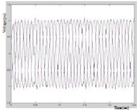
Figure 11. The output voltage mitigated by 12-pulse voltage-source converter STATCOM equipped with an RLC filter
