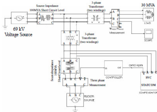
Figure 3. the studied power system
