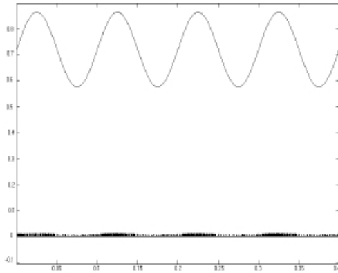
Figure 2: The instantaneous components of the 3-phase voltage flicker waveform
