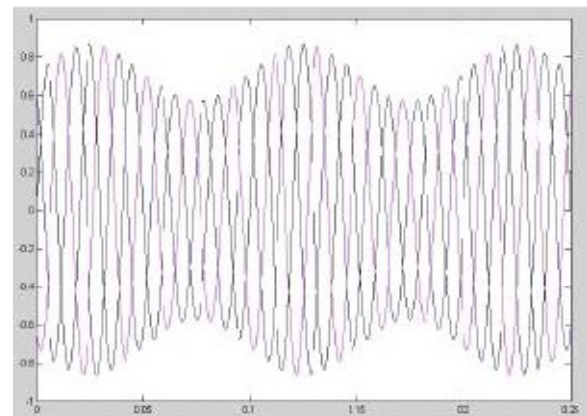
Figure 5. The generated voltage flicker by the flicker source
