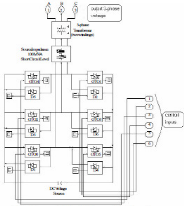
Figure 7. the circuit diagram of a 6-pulse voltage-source converter STATCOM
